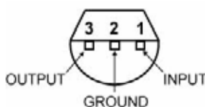
TO-92 (Z) (Bottom View)
